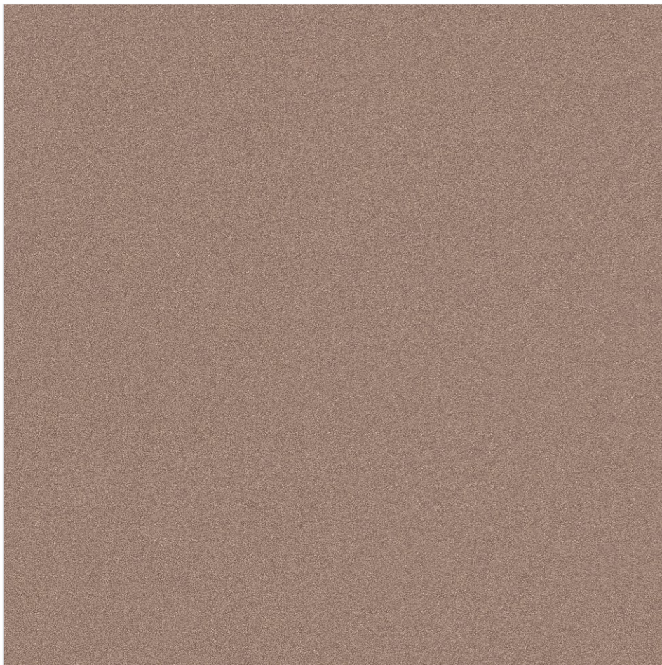
COPPER MATT
